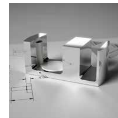
10.00S009.01 GUIADOR FIJO V-8MM INOX BRILLO FIXED GUIDE V-8MM POLISHED STAINLESS
